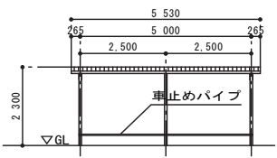
立面1/100
